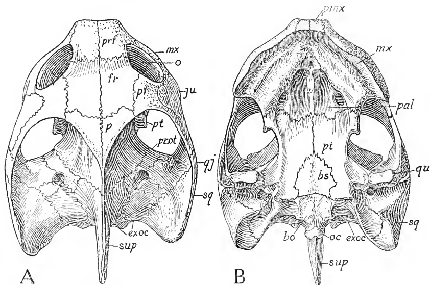
FIGURE 4.—Skull of Pseudemys idahoensis , U.S.N.M. No. 12059. Type. A, Superior view; B, inferior view. bo , Basioccipital; bs , basisphenoid; exoc , exoccipital; fr , frontal; ju , jugal; mx , maxillary; o , orbit; oc , occipital condyle; p , parietal; pal , palatine; pf , postfrontal; pmx , premaxillary; prf , prefrontal; pr. ot. , pro-otic; pt , pterygoid; qj , quadratojugal; qu , quadrate; sq , squamosal; sup , supraoccipital; r , vomer. Natural size
